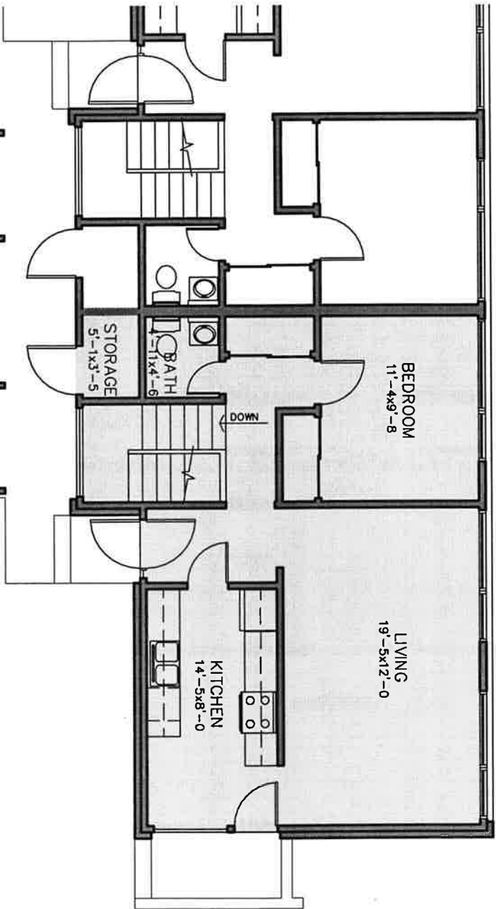
TYPE C3.2 PLAN
