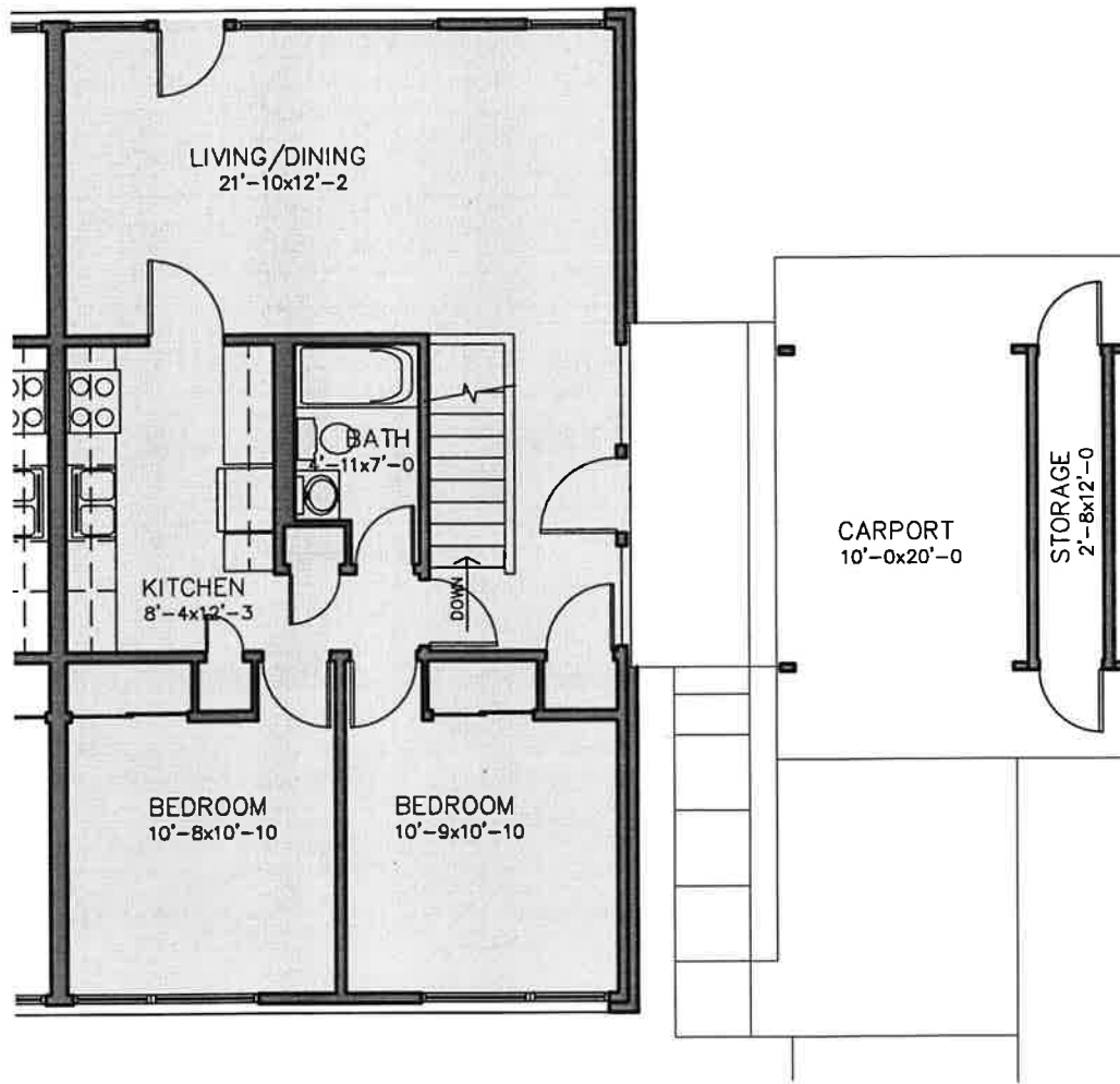
TYPE C1 FLOOR PLAN
